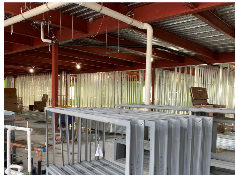
Installing interior studs in the 1st floor Area C.
